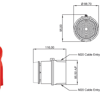
IS-SB Sounder Beacon
