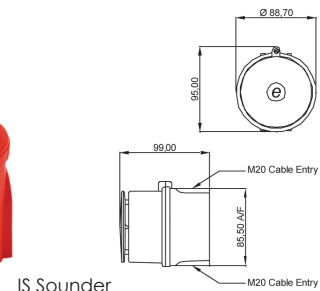
IS Sounder
