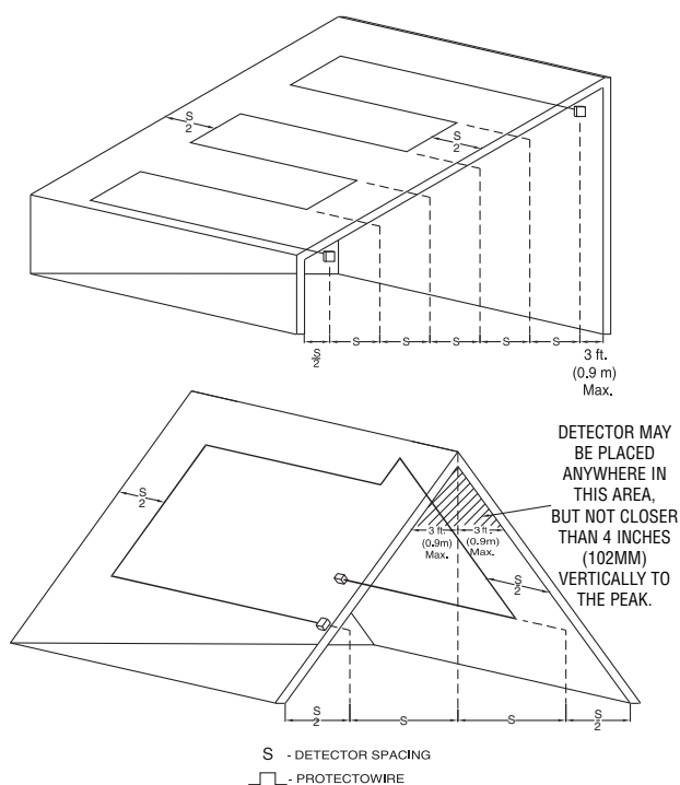
PROTECTOWIRE SPACING FOR SLOPED CEILINGS
