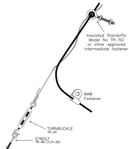
MESSANGER DETAIL RECOMMENDED FOR USE ON HIGH CEILINGS IN LARGE OPEN AREAS
