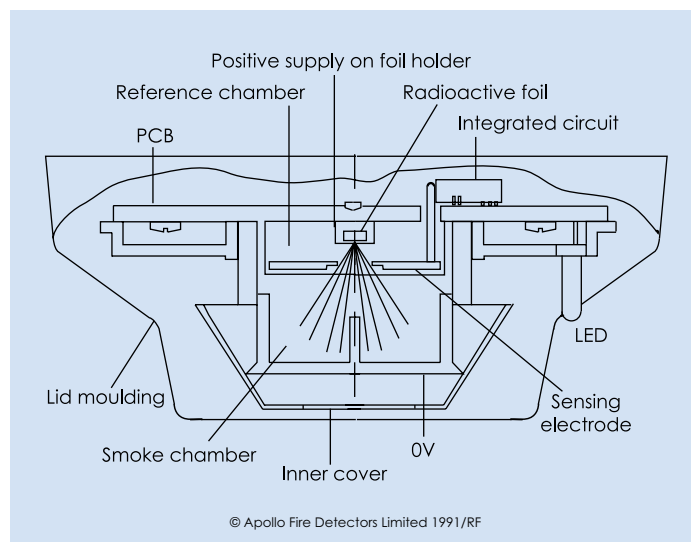
Fig.1 Side view, Series 65 Ionisation Smoke Detector
