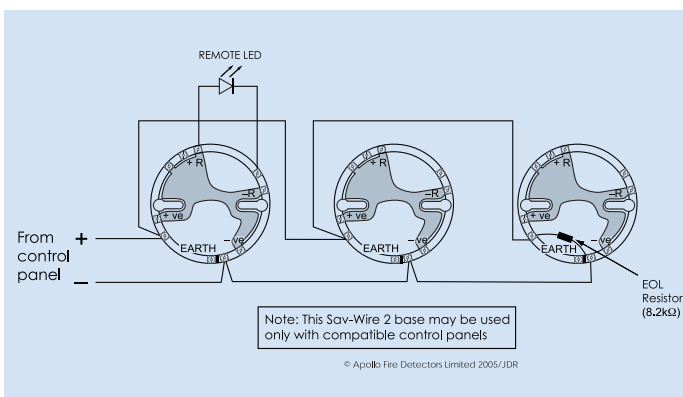
Fig.7 Wiring diagram of Sav-Wire Base
