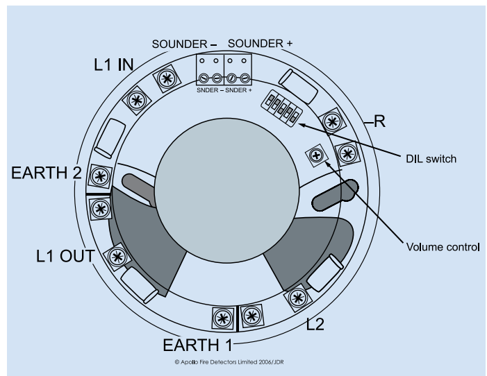
Fig.8 Wiring diagram of Series 65 Sounder Base
