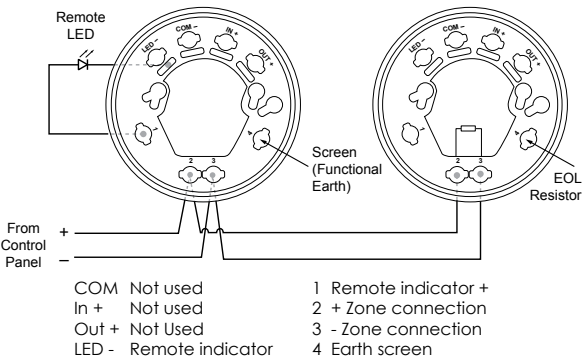
Sav-Wire base wiring connections
