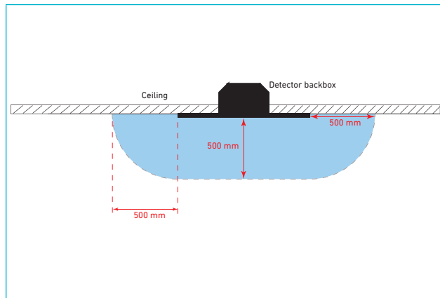
Figure 2: Overall minimum clearances
