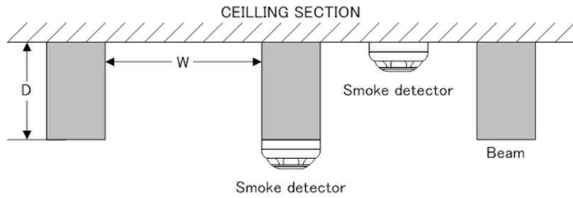
Figure 5: Smoke detector spacing — beam construction (side view)
