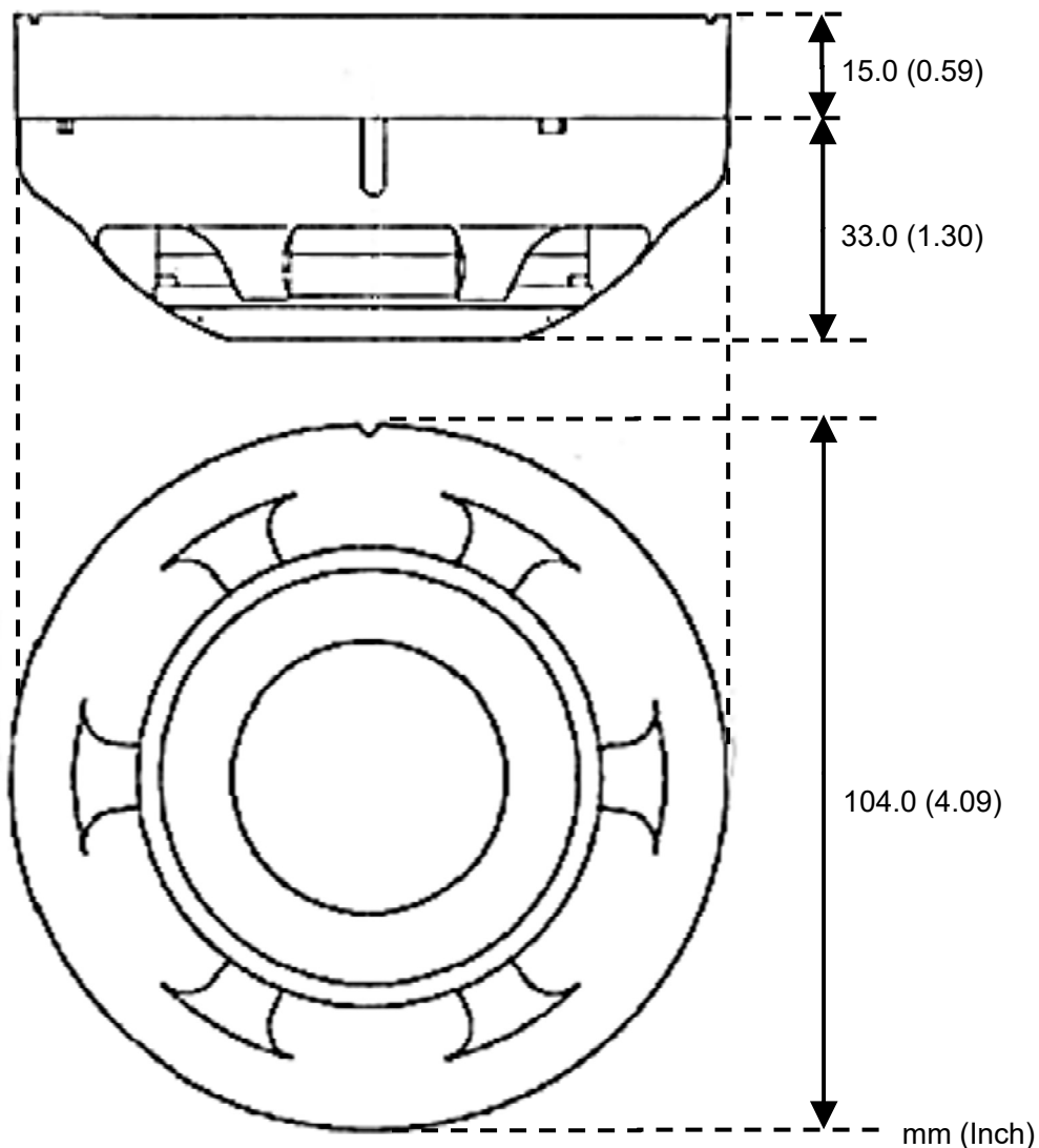
Figure1: Dimension of VDOT-PY
