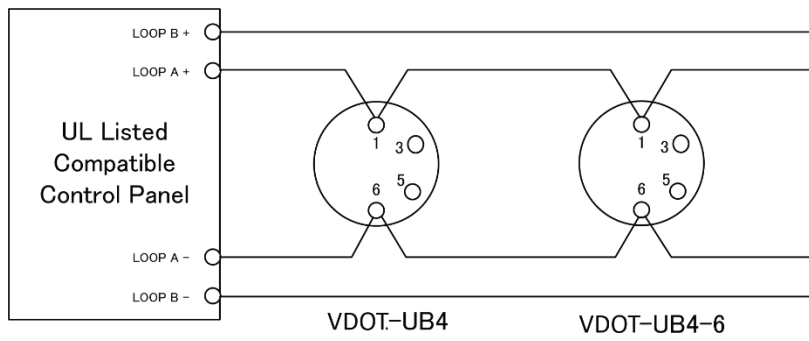
Figure 18: Wiring diagram for VDOT-UB4 and VDOT-UB4-6
