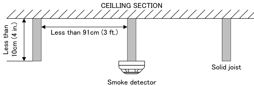
Figure 14: Smoke detector spacing — solid joist construction (side view)
