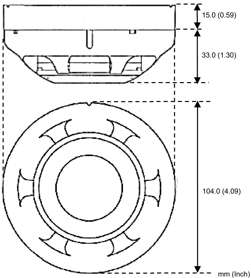
Figure 1: Dimension of VDOT-DPH
