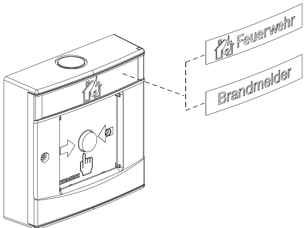
Figure 19: Attaching a self-adhesive sticker to the housing FDMH292-R
