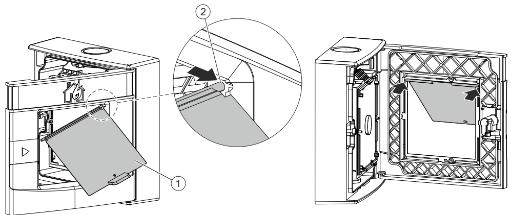
Figure 17: Example of installing protective cover DMZ1197-AC on a manual call point
