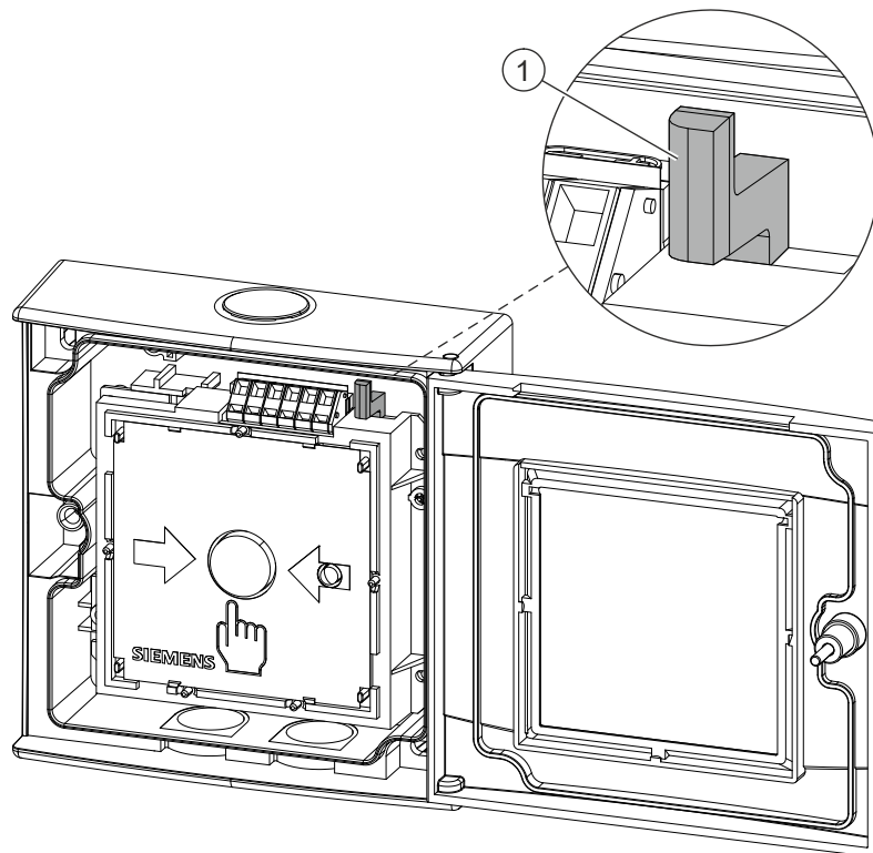
Figure 21: Resetting manual call point FDM223H
