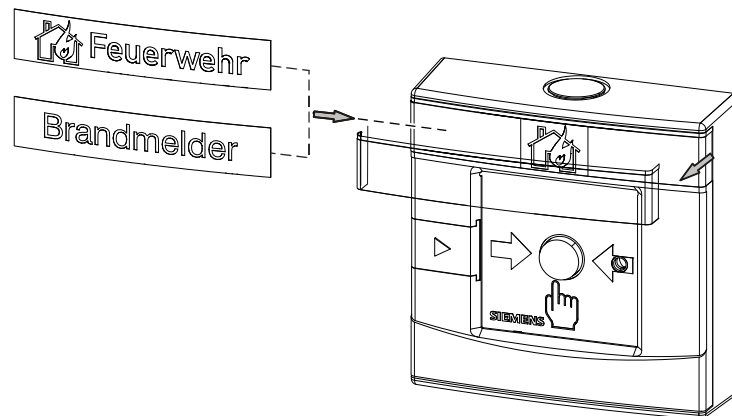
Figure 18: Attaching the stickers to a manual call point FDM223
