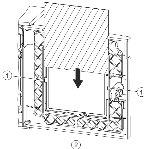
Figure 22: Replacing the glass insert
