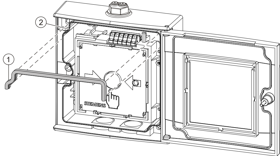
Figure 16: Mounting the seal FDMP223
