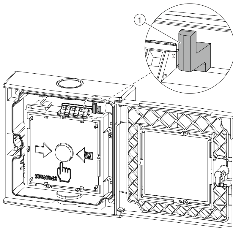
Figure 20: Resetting manual call point FDM223
