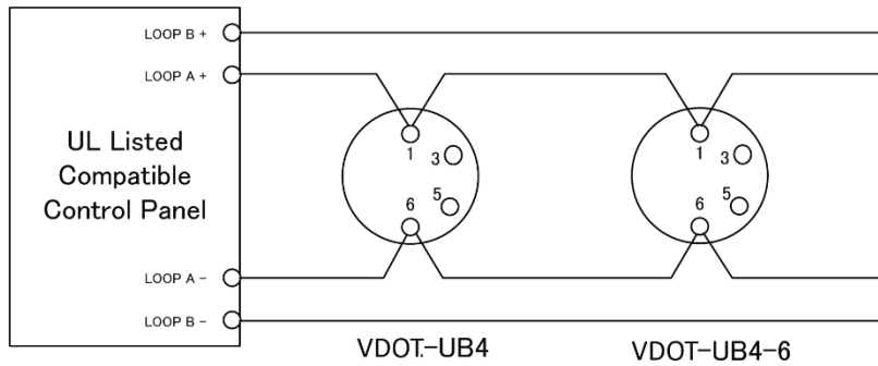
Figure 13: Wiring diagram for VDOT-UB4 and VDOT-UB4-6
