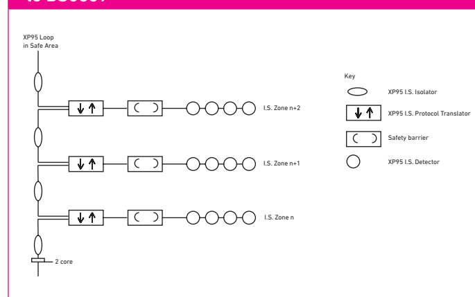
Figure 1: Schematic wiring diagram of XP95 I.S. circuit to BS5839
